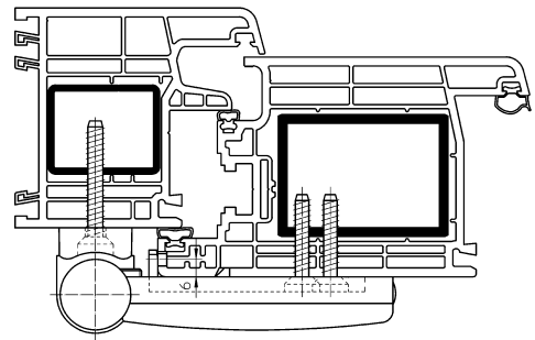
cross section
